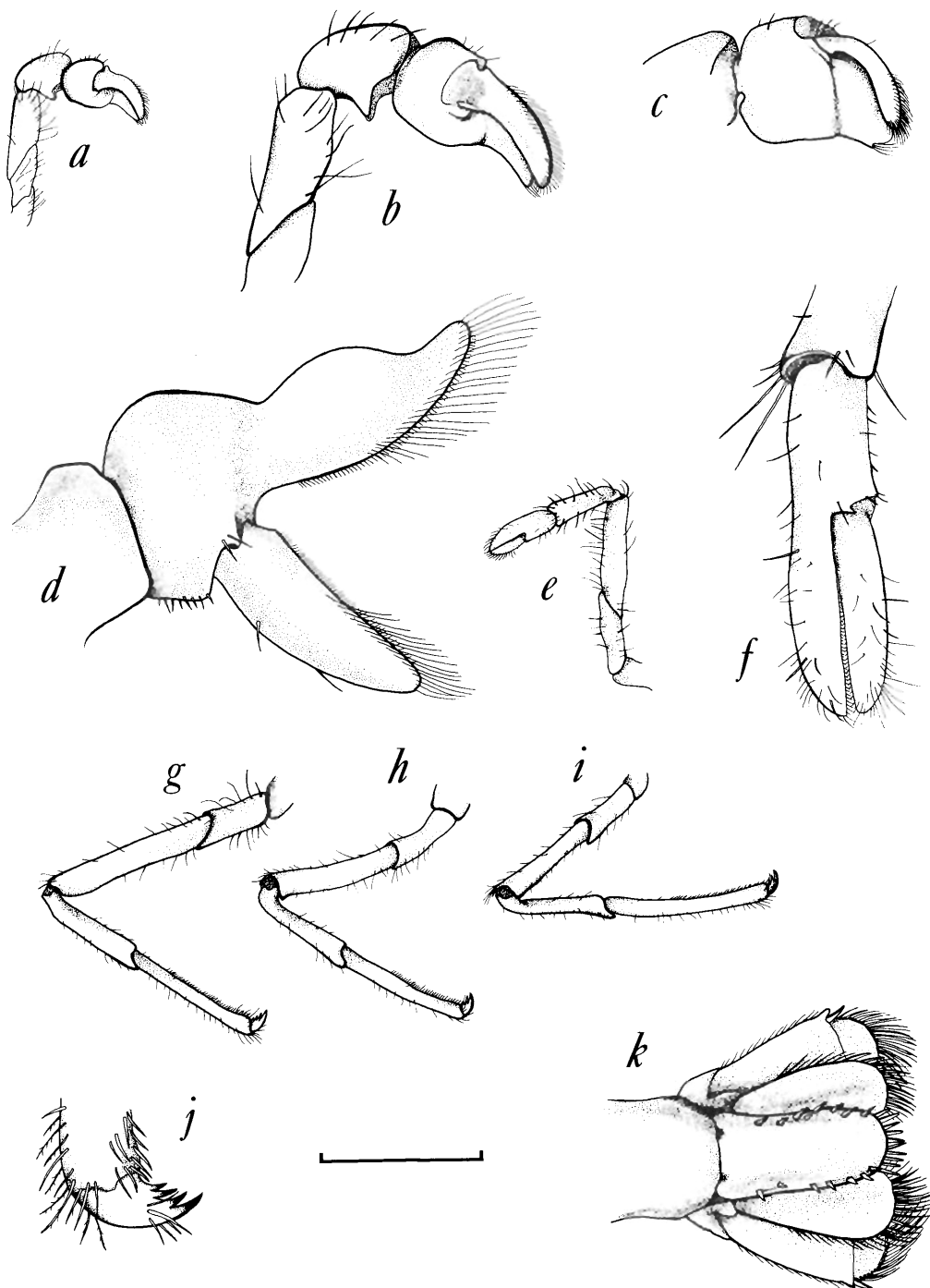
Fig. 3. Chorocaris fortunata , female holotype (except a-c), pereiopods and telson. a, right chela of female paratype of similar size as holotype (CL 8.7 mm) (right cheliped regenerating in holotype); b, higher magnification of same chela seen in a; c, inner surface of same chela shown in a and b; d, left chela, turned to expose indentations on outer face of propodus; e, second pereiopod; f, chela of second pereiopod (note relative lengths of dactylus and propodus); g-i, pereiopods 3-5; j, dactylus of pereiopod 3 (from figure g); k, dorsal view of telson and uropods. Scale bar = 4.2 mm (a, e, g-i, k); 2.0 mm (b, c); and 1.0 mm (d, f, j).
