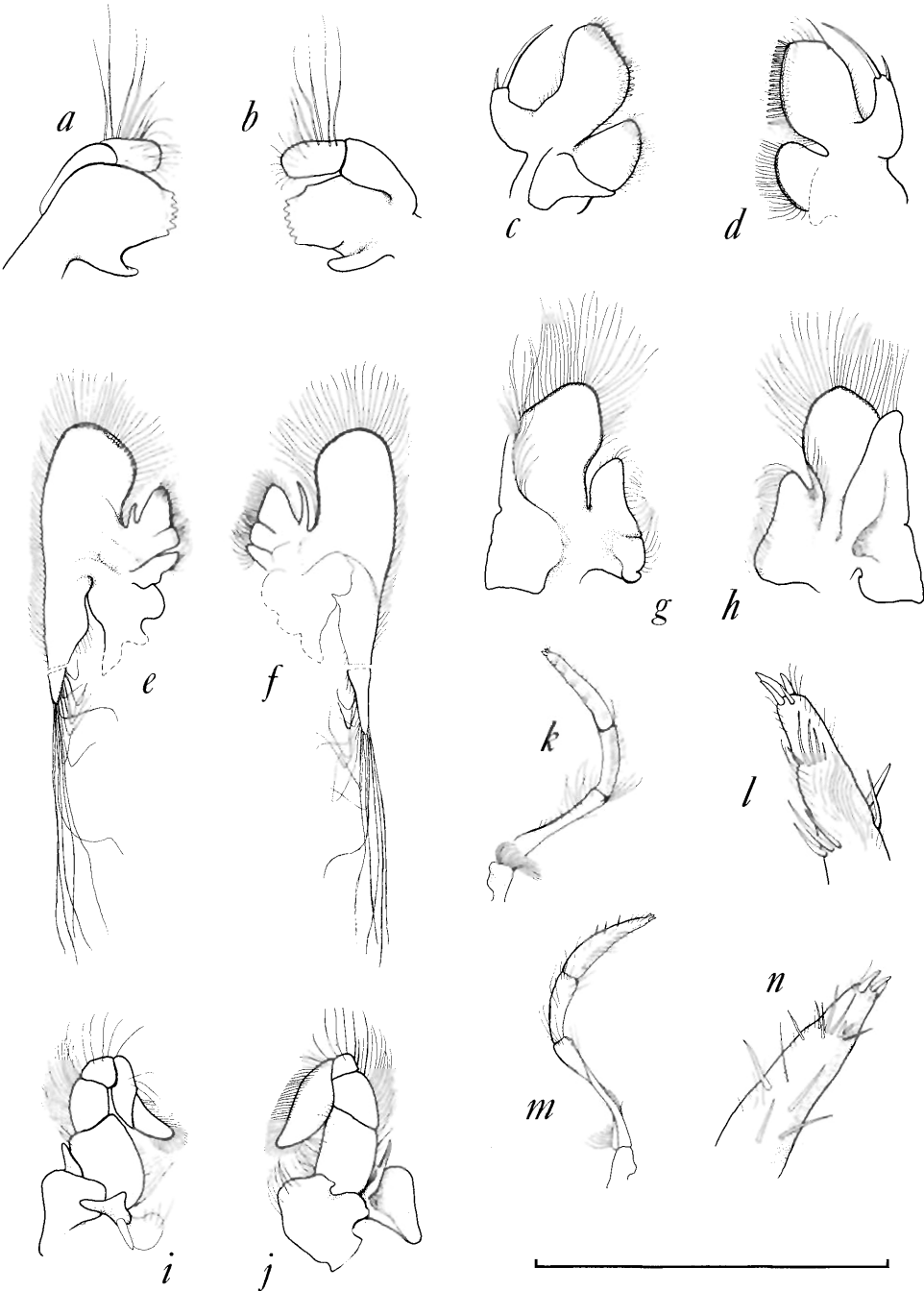
Fig. 2. Chorocaris fortunata , female holotype, mouthparts. a, b, right mandible in outer (a) and inner (b) view; c, d, right first maxilla in outer (c) and inner (d) view; e, f, right second maxilla in outer (e) and inner (f) view; lower part of figures e and f (area with long setae, below dotted line on basal region of exopod) taken from female paratype of similar size to holotype (CL 8.7 mm) (missing on right maxilla of holotype); g, h, right third maxilliped in outer (g) and inner (h) view; i, j, right second maxilliped in outer (i) and inner (j) view; k, l, m, and n, third maxilliped, outer view with higher magnification of tip (k, l) and inner views of same (m, n). Scale bar = 2.5 mm (a-d, l, n); 5.0 mm (e-j), and 10.4 mm (k, m).
